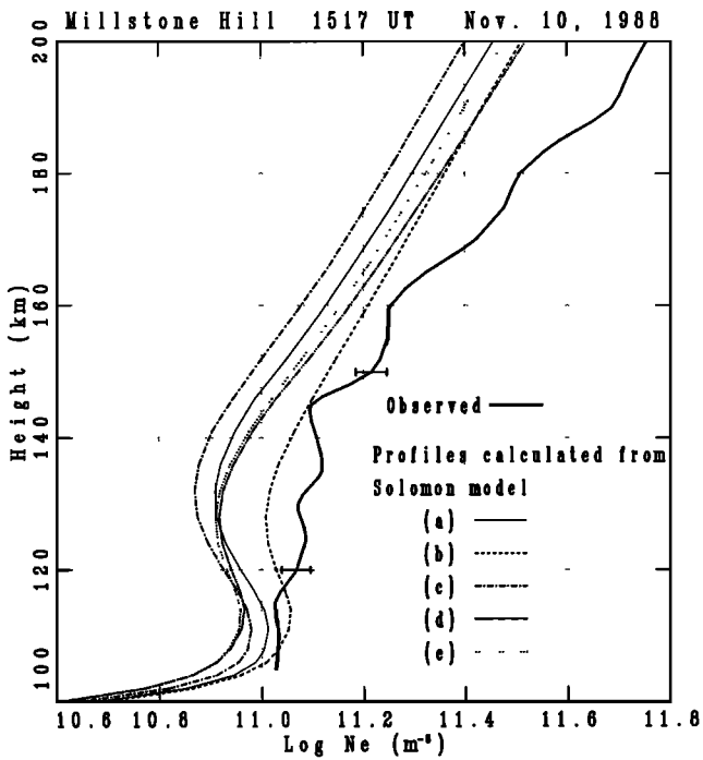
Fig. 4. Electron density profiles at Millstone Hill for 1517 UT (1031 LMT) on November 10, 1988. Heavy solid line: observed incoherent scatter profile. Key for EUV flux models used in profiles calculated with the Solomon photochemical model: (a) Hinteregger et al. [1981] model; (b) Hinteregger et al. model except that fluxes at wavelengths less than 250 Å have been doubled; (c) Linear interpolation using F10.7 between SC#21REFW and F79050N reference spectra; (d) Tobiska [1991] model; (e) rocket flight measurements [Woods and Rottman, 1990].
