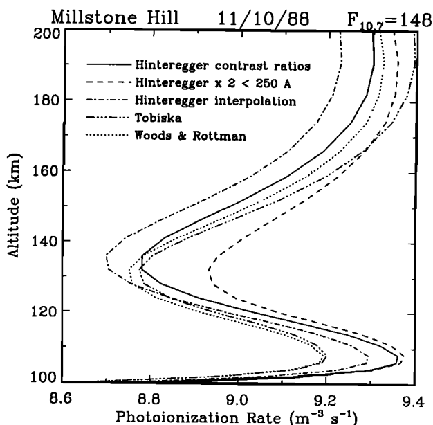
Fig. 2. Photoionization rates calculated using the Solomon model for five solar flux cases and 1517 UT on November 10, 1988, at Millstone Hill (log units).
