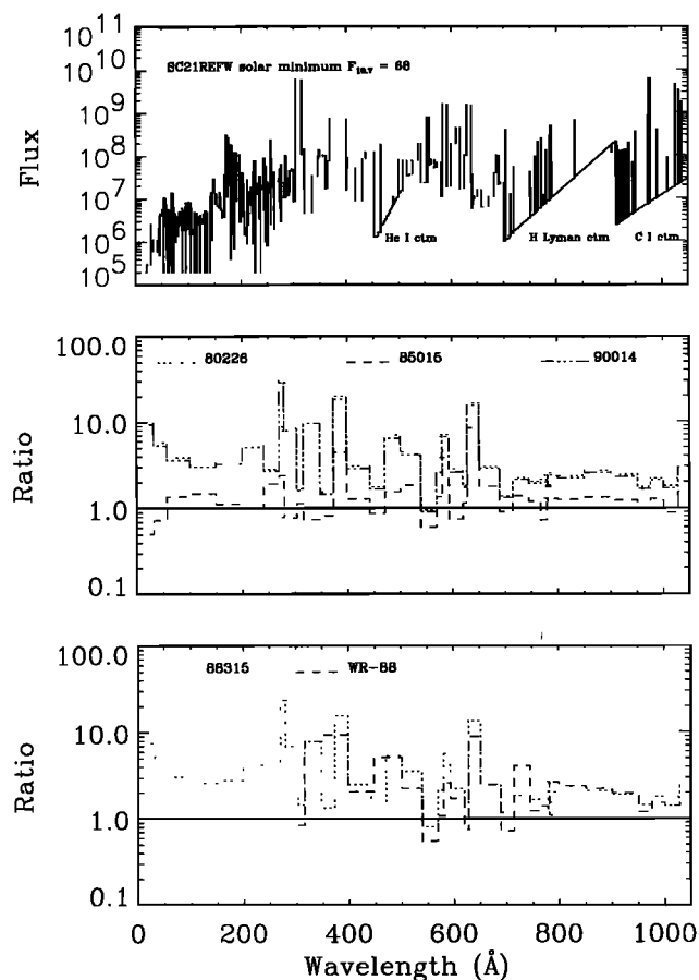
Fig. 1. The solar spectra for the Tobiska [1991] model compared to the SC#21REFW spectrum [Hinteregger et al., 1981] in 39 wavelength intervals between 18 and 1050 Å. The top panel shows the high resolution reference spectrum for solar cycle 21 minimum when F_{10.7} = 68 . The middle and bottom panels show the ratio of the Tobiska EUV model spectra to SC#21REFW where each model spectrum on a given date is denoted by a differently labeled line. Day 226 of 1980 is 80226, while WR-88 is the November 10, 1988, Woods and Rottman [1990] spectrum.
