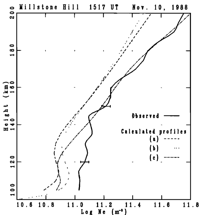
Fig. 8. Electron density profiles at Millstone Hill for 1517 UT (1031 LMT) on November 10, 1988. Heavy solid line: observed incoherent scatter profile. Key for calculated profiles: (a) revised Buonsanto photochemical model; (b) Solomon photochemical model; (c) revised Buonsanto photochemical model with MSIS-86 [N 2 ] and [O 2 ] multiplied by 0.5.
