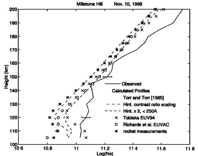
Figure 5. Same as Figure 3, except for 1517 UT (1047 LST) on November 10, 1988, and one additional profile is shown which was obtained using the EUV fluxes from sounding rocket measurements [Woods and Rottman, 1990] on that day input to the model.
