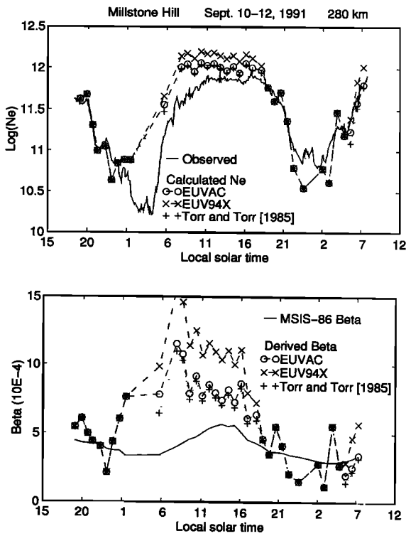
Figure 13. Observations and results of the Millstone Hill semiempirical ionospheric model for a fixed height of 280 km on September 10–12, 1991. (top) Millstone Hill radar electron density measurements, together with calculated electron density for three different EUV flux models. (bottom) The O^+(^4S) recombination rate \beta calculated from the MSIS-86 model using equation (5), and derived from the incoherent scatter data and the modeled production rates using the three EUV flux models and equation (4).
