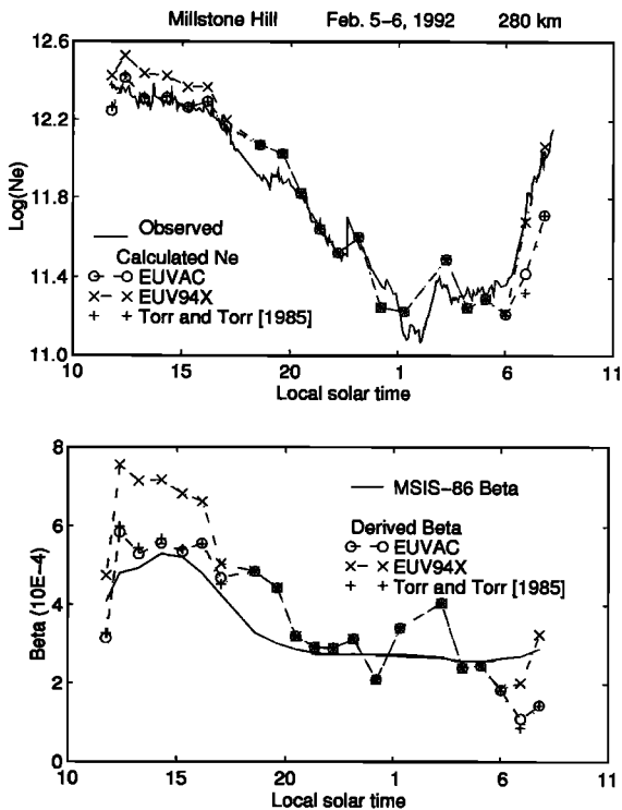
Figure 14. Same as Figure 13, except for February 5–6, 1992.
