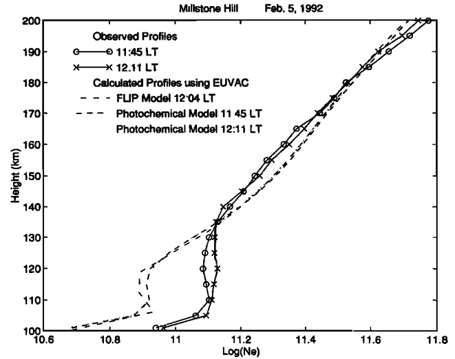
Figure 8. Electron density profiles at Millstone Hill near noon on February 5, 1992. Two incoherent scatter profiles are shown, together with results from both the Millstone Hill ionospheric model and the FLIP model. For the simulations from both ionospheric models the EUVAC solar flux model was used.
