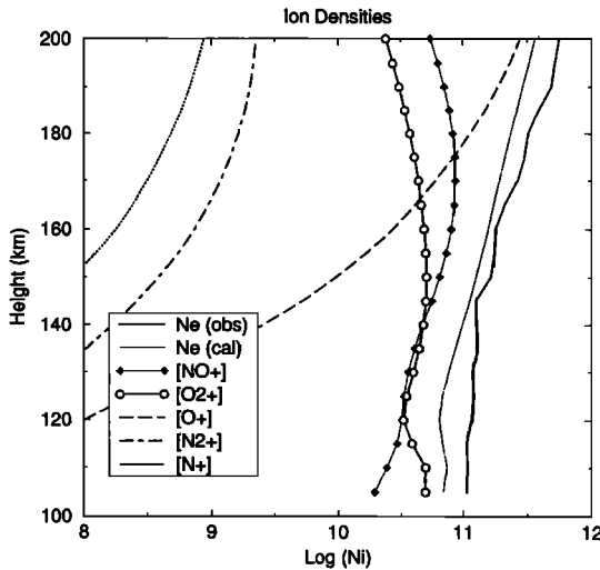
Figure 7. Ion density profiles calculated for 1517 UT (1047 LST) on November 10, 1988, using the rocket measurements as input to the Millstone Hill ionospheric model. Cross sections based on [Fennelly and Torr, 1992] and pel/pi ratios obtained from the GLOW model were used.
