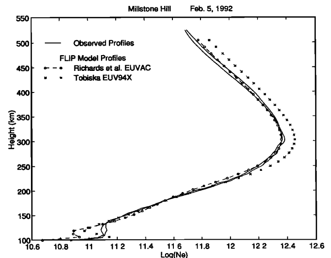
Figure 12. The observed and FLIP model electron density profiles of Figures 8 and 9 extended upward into the topside of the F2 region.
