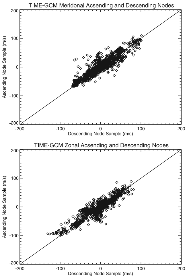
Figure 5. The comparisons between ascending and descending nodes of the TIDI sampled TIME-GCM meridional and zonal winds at 90 km ( 60\text{--}52^\circ\text{N} ). The good agreements show that the zonally averaged neutral winds at same local time and latitude are roughly the same, even they are sampled a few days apart.
