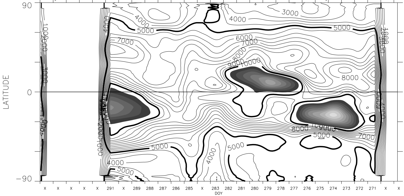
1.20 R sun version 1 cal + Feb 2002 opal cor. pB units : 1.0e-10 B sun
