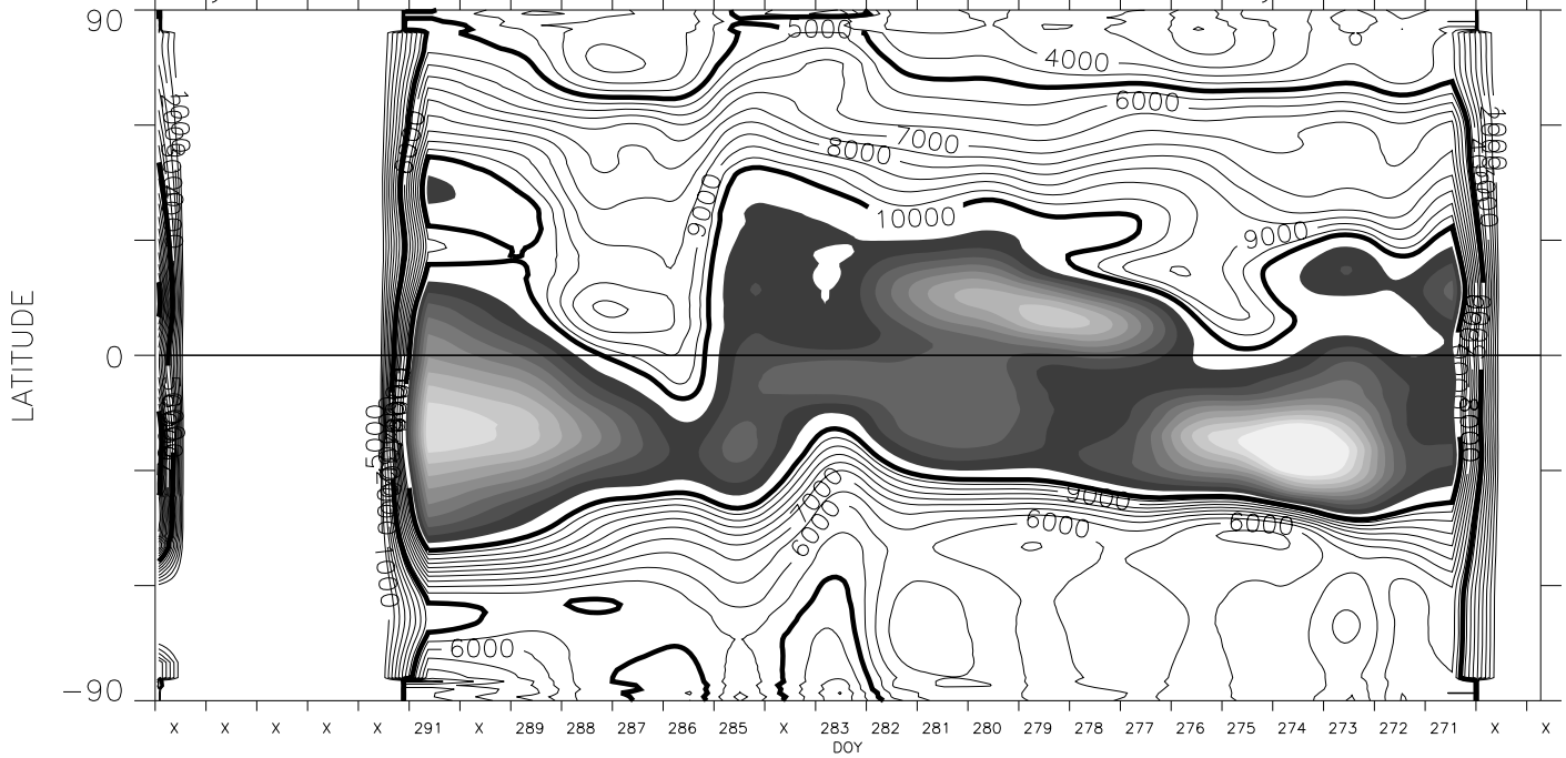
1.15 R sun version 1 cal + Feb 2002 opal cor. pB units : 1.0e-10 B sun
