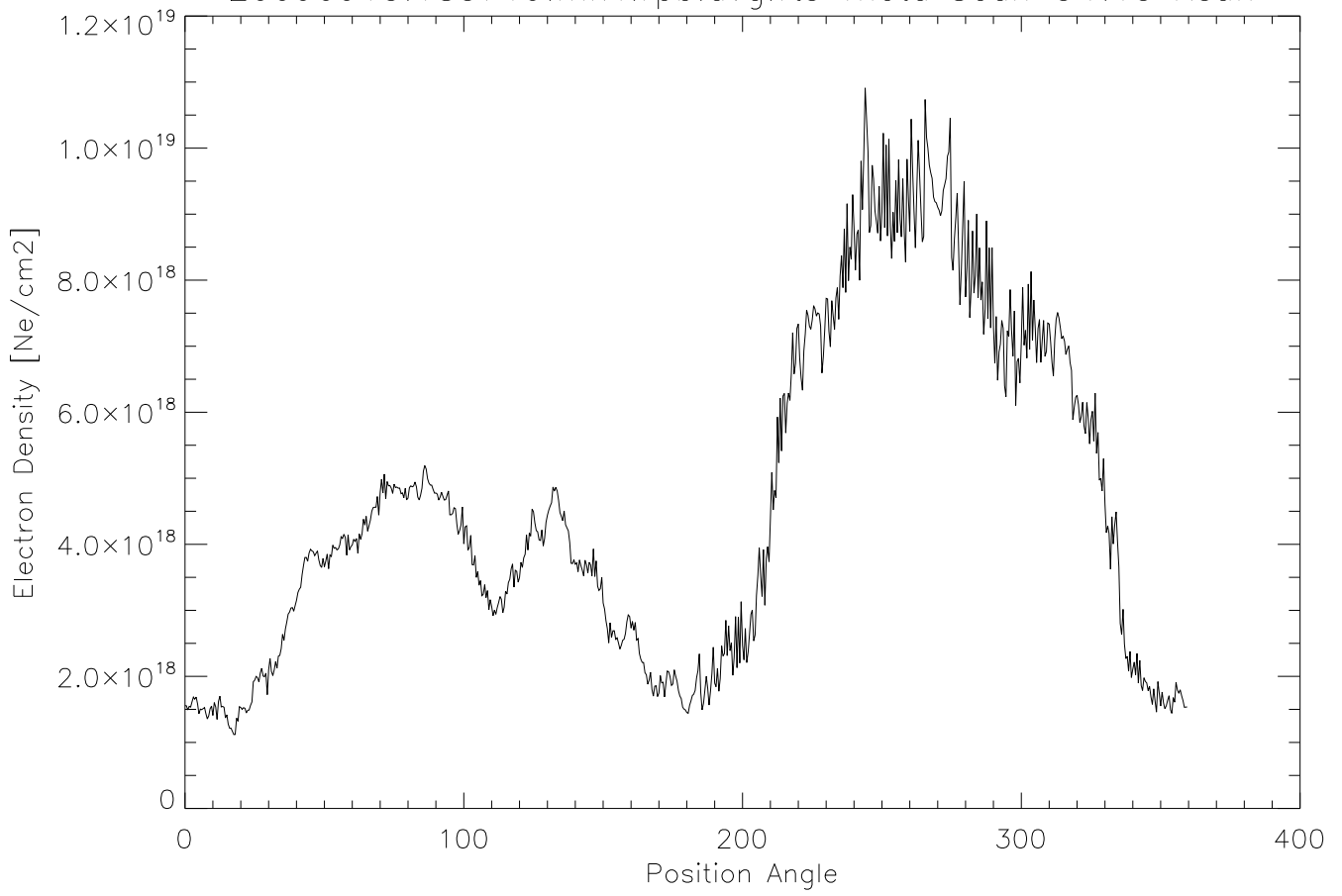
20090915.185719.mk4.rpb.avg.fts Theta Scan @1.15 R sun
