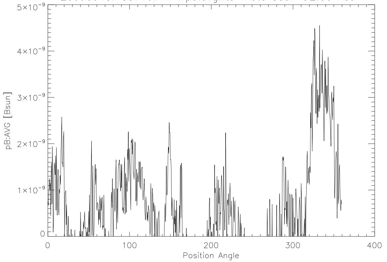
20090915.185719.mk4.rpb.avg.fts Theta Scan @2.50 R sun
