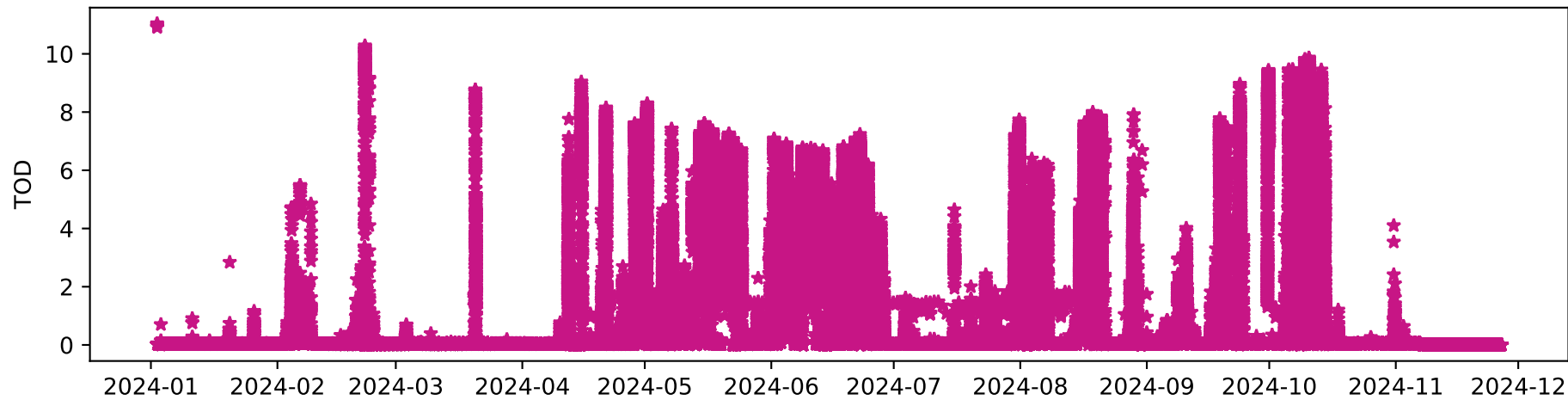
total optical depth
